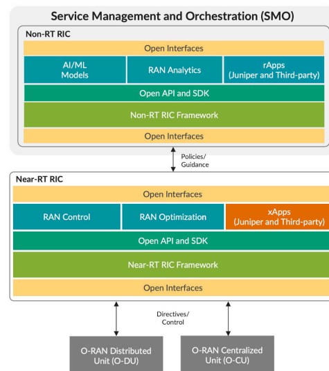
Figure 1: Juniper RIC is fully compliant with O-RAN specifications and interfaces, supporting both an open API and SDK for integration with third-party xApps and rApps.
